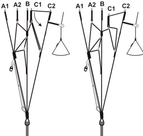
Fig. 9 Adjustment of flightdirection by C-bridge
