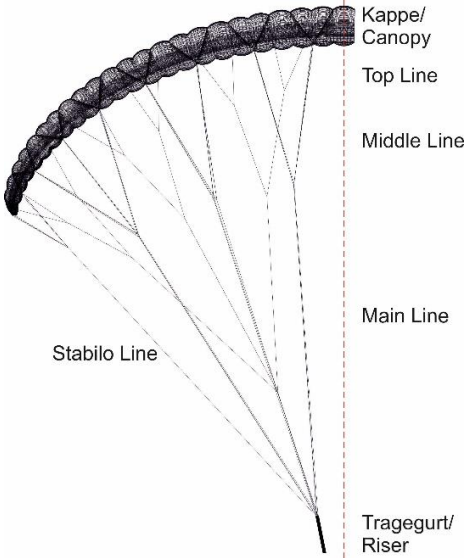
Fig. 1 CAD drawing of AGERA RS
