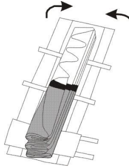
Fig. 13 The glider is now folded up along its length, and the leading edges are on top of each other without having being bent.
